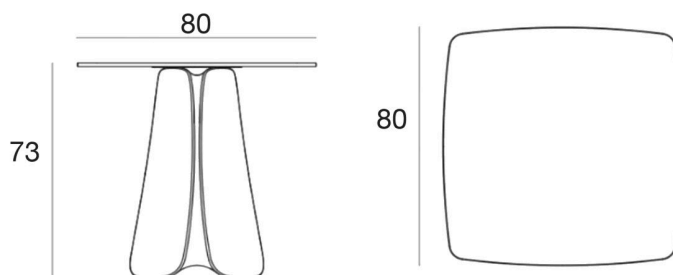
80 × 80 × 73 cm
